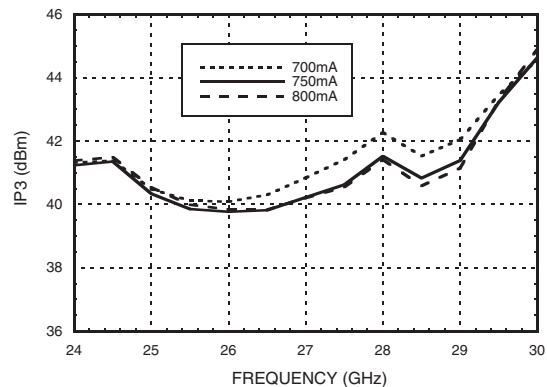
Output IP3 vs. Supply Current, Pout/Tone = +19 dBm
